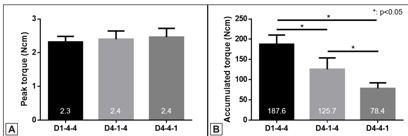
Figure 4. Peak and accumulated drilling torque values for the three bone density distribution models.
