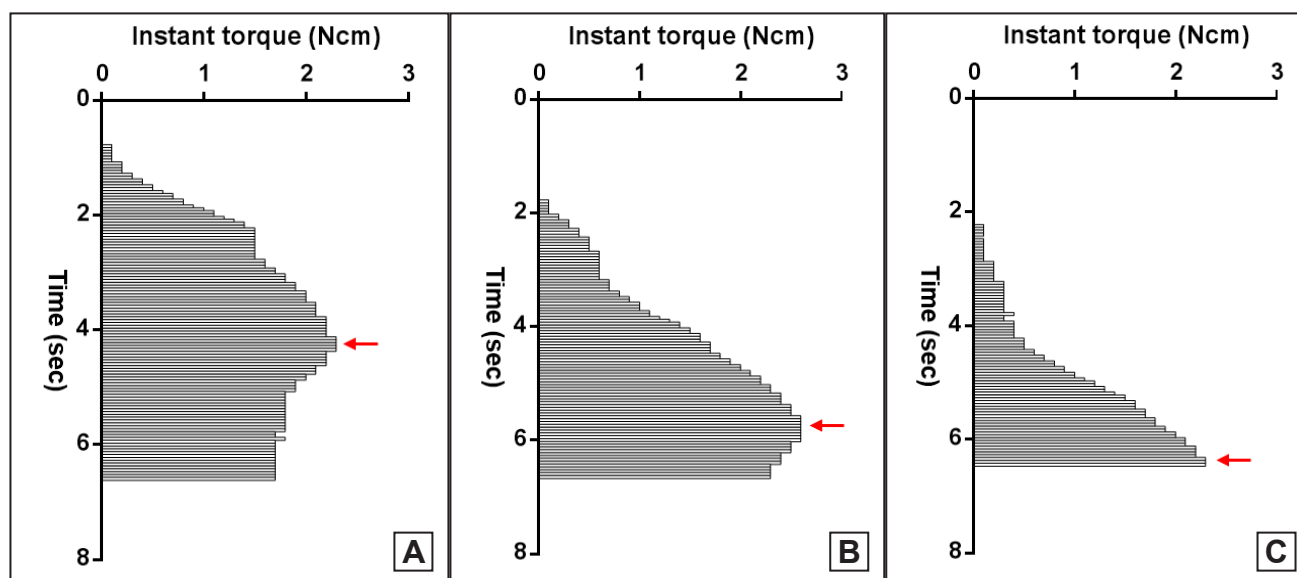
Figure 3. Representative drilling torque profiles for the three bone density distribution models.
