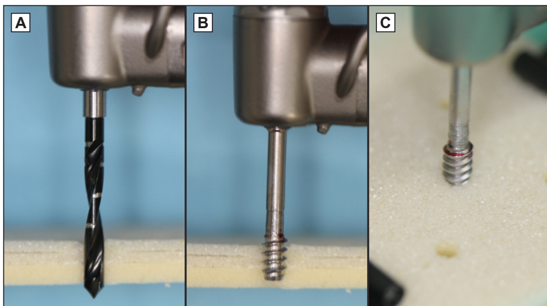
Figure 2. Experimental procedure: A = initial osteotomy preparation using a 2.0-mm twist drill; B = drilling using the 2.7-mm torque-measurement drill; C = torque measurement during drilling.
